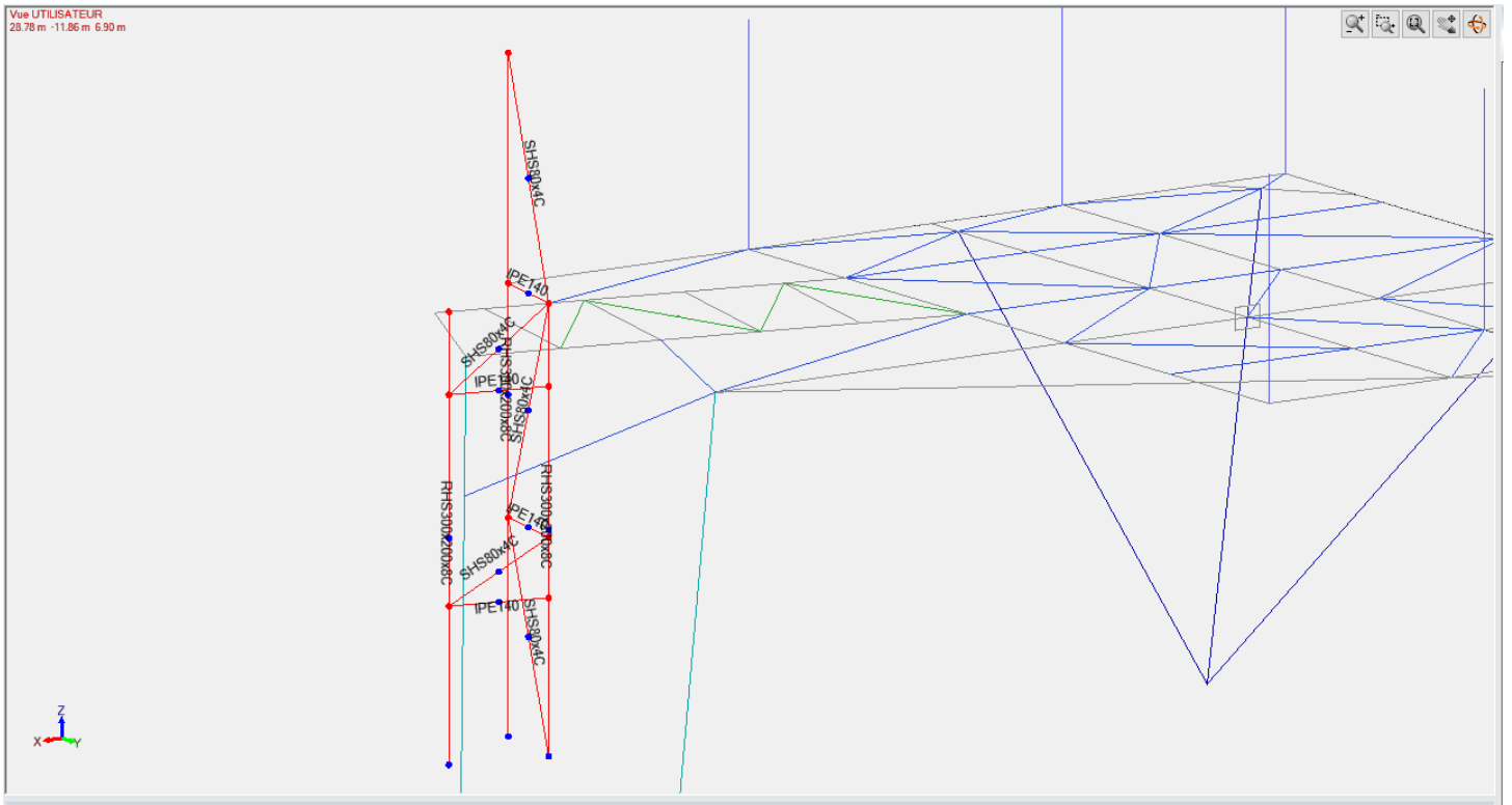
Structure autour pylône ascenseur, poteau tube R300x200x8, lisses IPE140, Diag TC80x4
