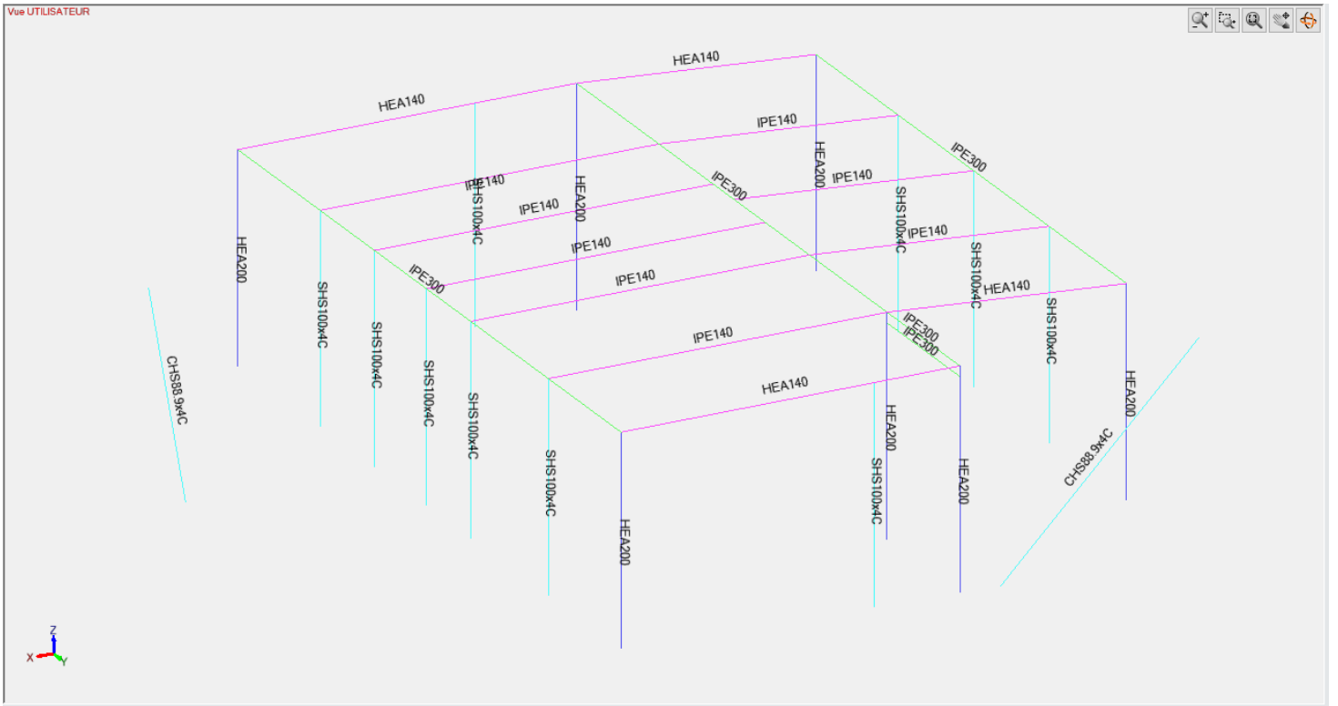
Poteaux, poutres, pannes, potelets façade et potelets BS
